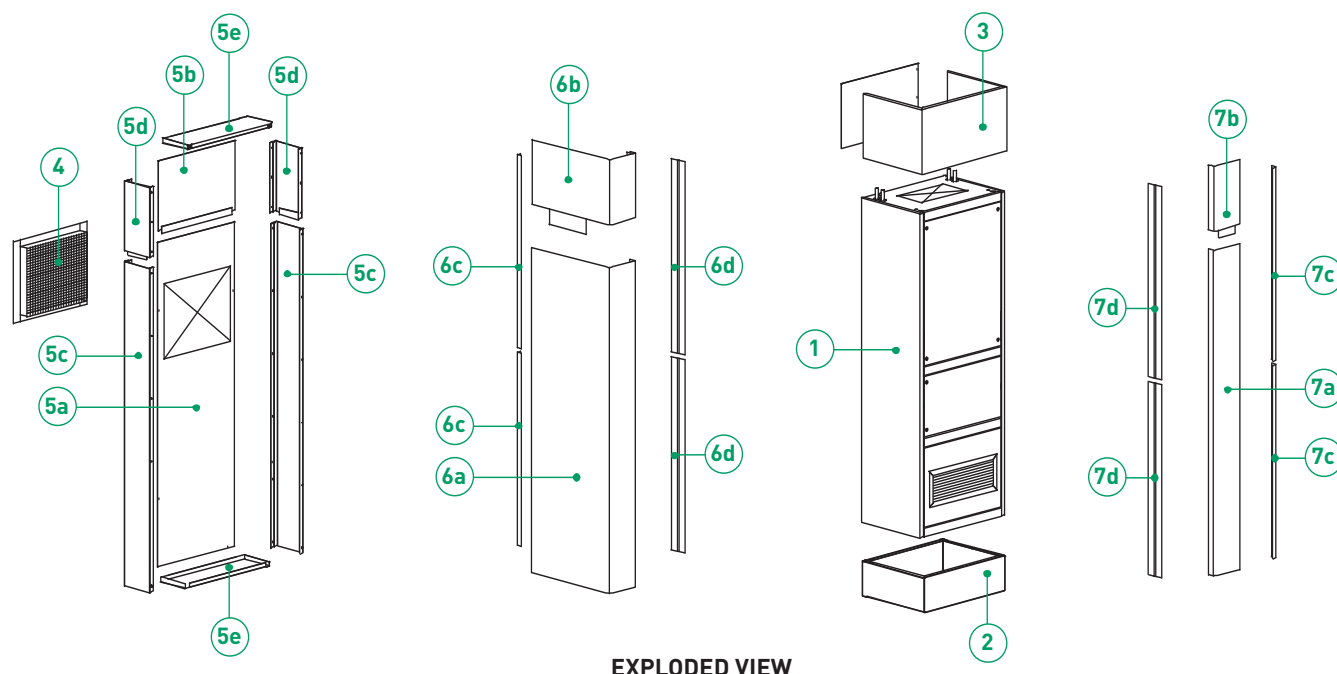
EXPLODED VIEW
