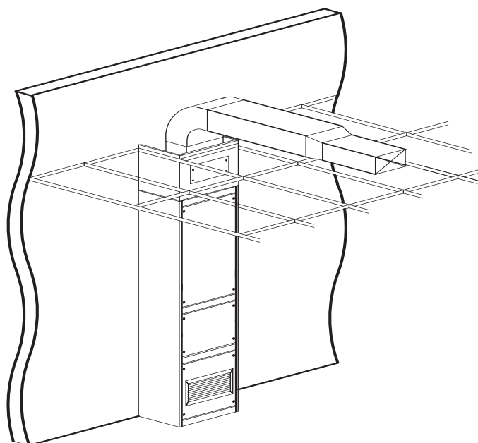
FINAL ASSEMBLY VIEW
