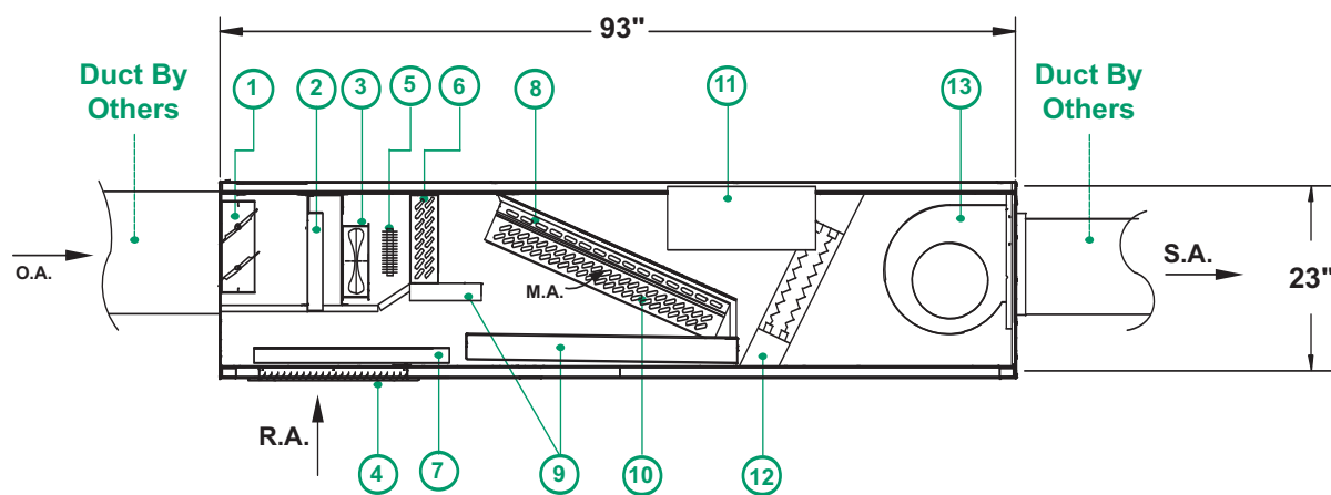
SIDE SECTION
