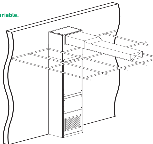
FINAL ASSEMBLY VIEW
