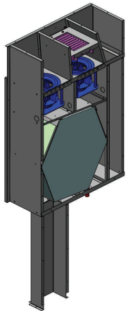
TR Recovery Module
