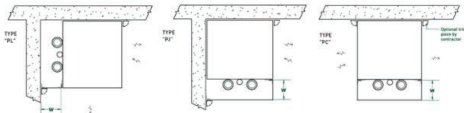
One, Two, and Three-Sided Pipe Cover/Block-Off Options
