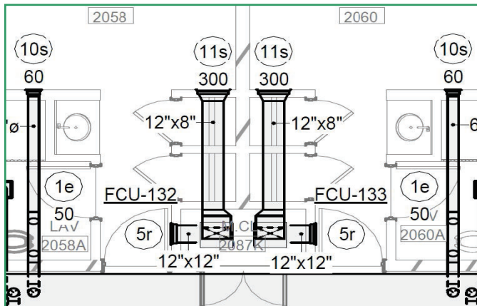
Figure 3: Dormitory with mechanical closet and ducted return
