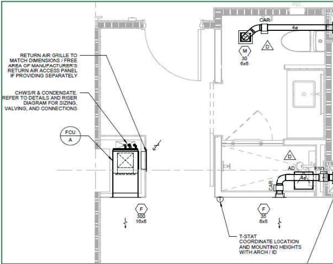
Figure 1: Hotel with low ceiling, ducted supply, and front return
