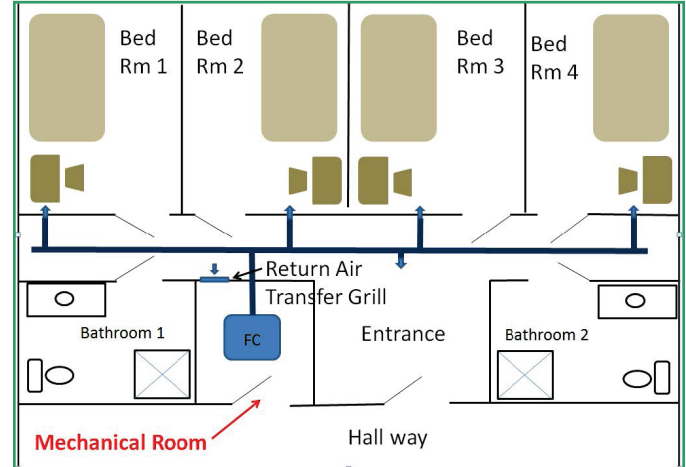
Figure 2: Dormitory with mechanical closet and plenum return
